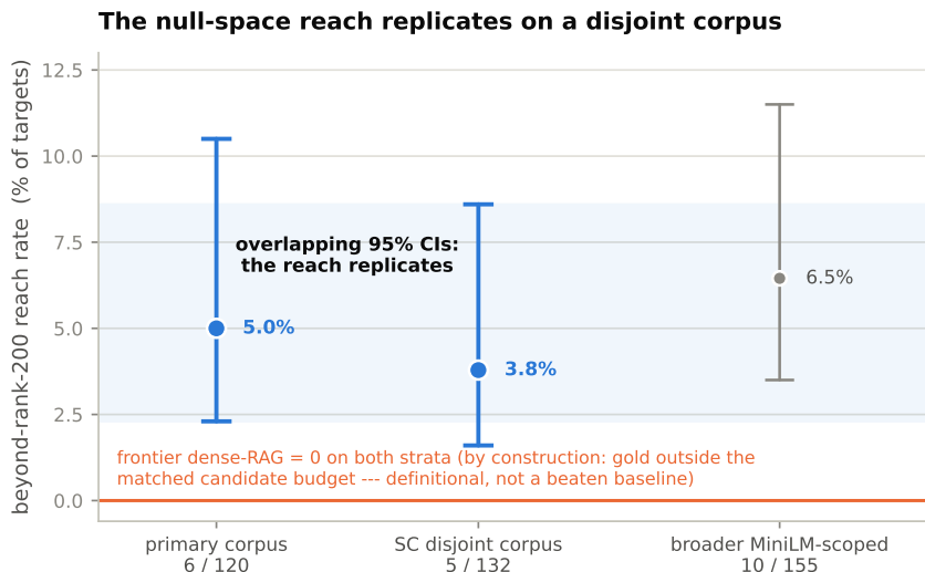
Figure 8: Second-corpus replication of the null-space reach. Beyond-rank-200 reach rate with Wilson 95% intervals on the primary corpus (6 of 120, [2.3, 10.5]%) and the fully disjoint second corpus (5 of 132, [1.6, 8.6]%), substrate arm; the broader MiniLM-scope figure (10 of 155, [3.5, 11.5]%) is shown lighter for context. The overlapping intervals are the replication claim. Frontier dense-RAG sits at 0 on both strata by construction (the stratum is defined as gold outside the matched candidate budget), so the 0 is definitional, not a beaten baseline; the substrate-versus-RAG McNemar p = 0.0625 is descriptive, not significant. The second corpus is an independent target and gold-source harvest scored over the shared source pool: the replication is on disjoint targets and gold, and independent-pool generalisation remains untested.
