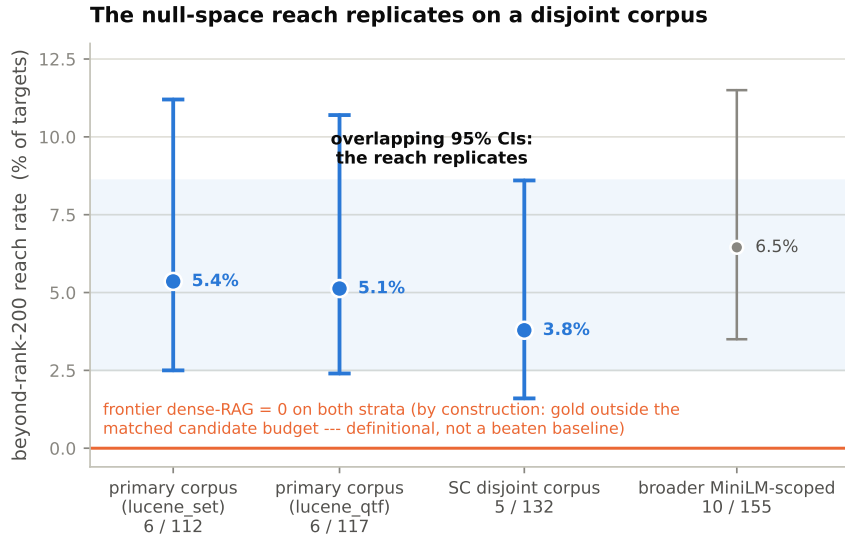
Figure 8: Second-corpus replication of the null-space reach. Beyond-rank-200 reach rate with Wilson 95% intervals on the primary corpus, plotted as one point per stratum convention (6 of 112, [2.5, 11.2]% under lucene_set ; 6 of 117, [2.4, 10.7]% under lucene_qtf , both counts independently re-derived and confirmed) and the fully disjoint second corpus (5 of 132, [1.6, 8.6]%), substrate arm; the broader MiniLM-scoped figure (10 of 155, [3.5, 11.5]%) is shown lighter for context. The overlapping intervals are the replication claim. Frontier dense-RAG sits at 0 on both strata by construction (the stratum is defined as gold outside the matched candidate budget), so the 0 is definitional, not a beaten baseline; the substrate-versus-RAG McNemar p = 0.0625 is descriptive, not significant. The second corpus is an independent target and gold-source harvest scored over the shared source pool: the replication is on disjoint targets and gold, and independent-pool generalisation remains untested.
